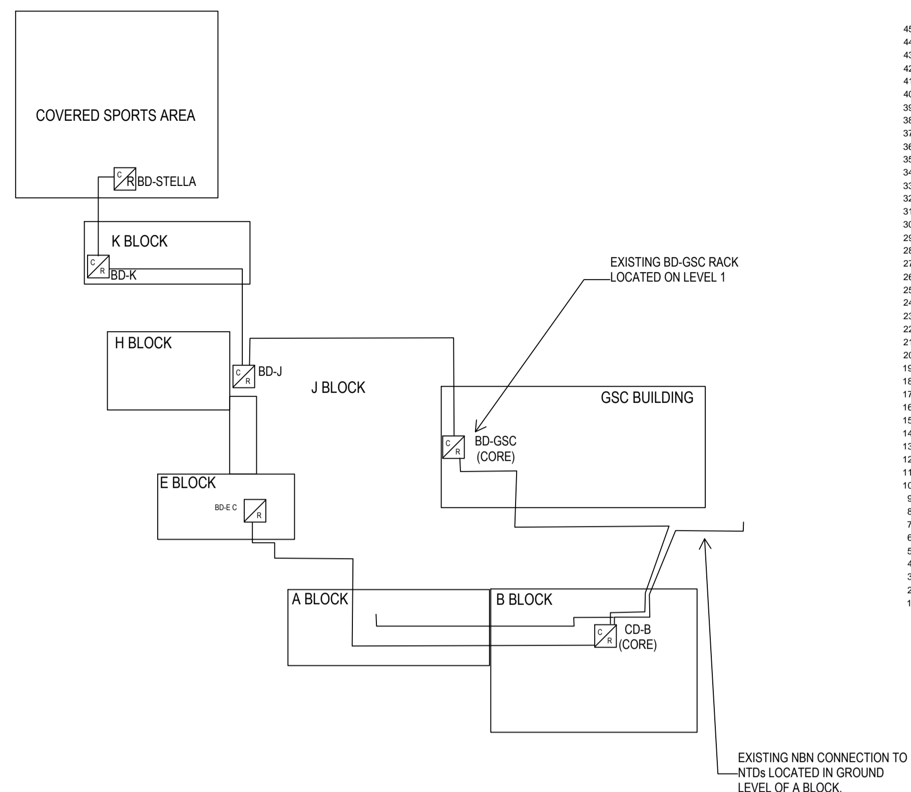
EXISTING OPTICAL FIBRE COMMUNICATIONS SCHEMATIC
