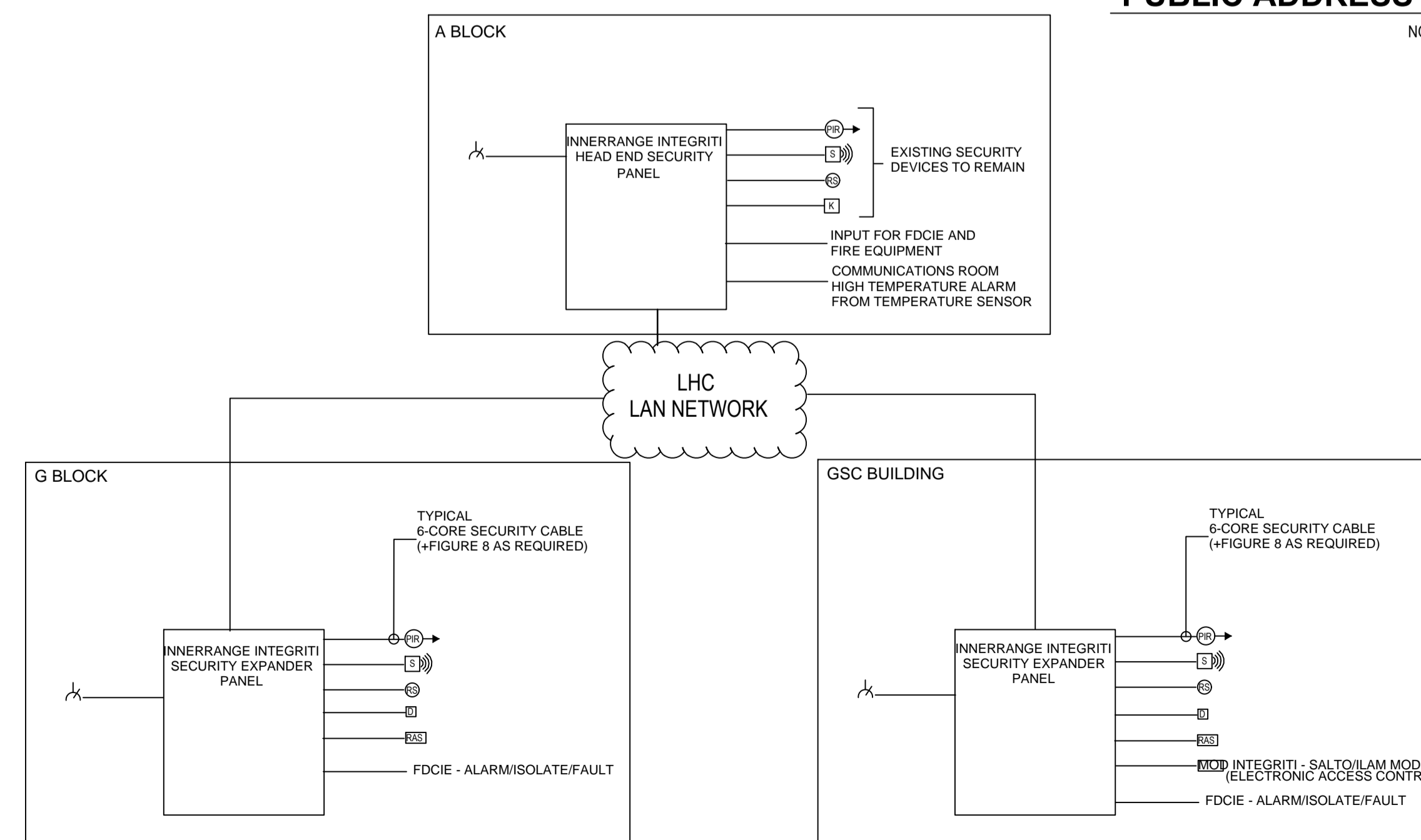
SECURITY ALARM SCHEMATIC
