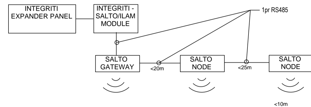
ELECTRONIC ACCESS CONTROL SCHEMATIC
