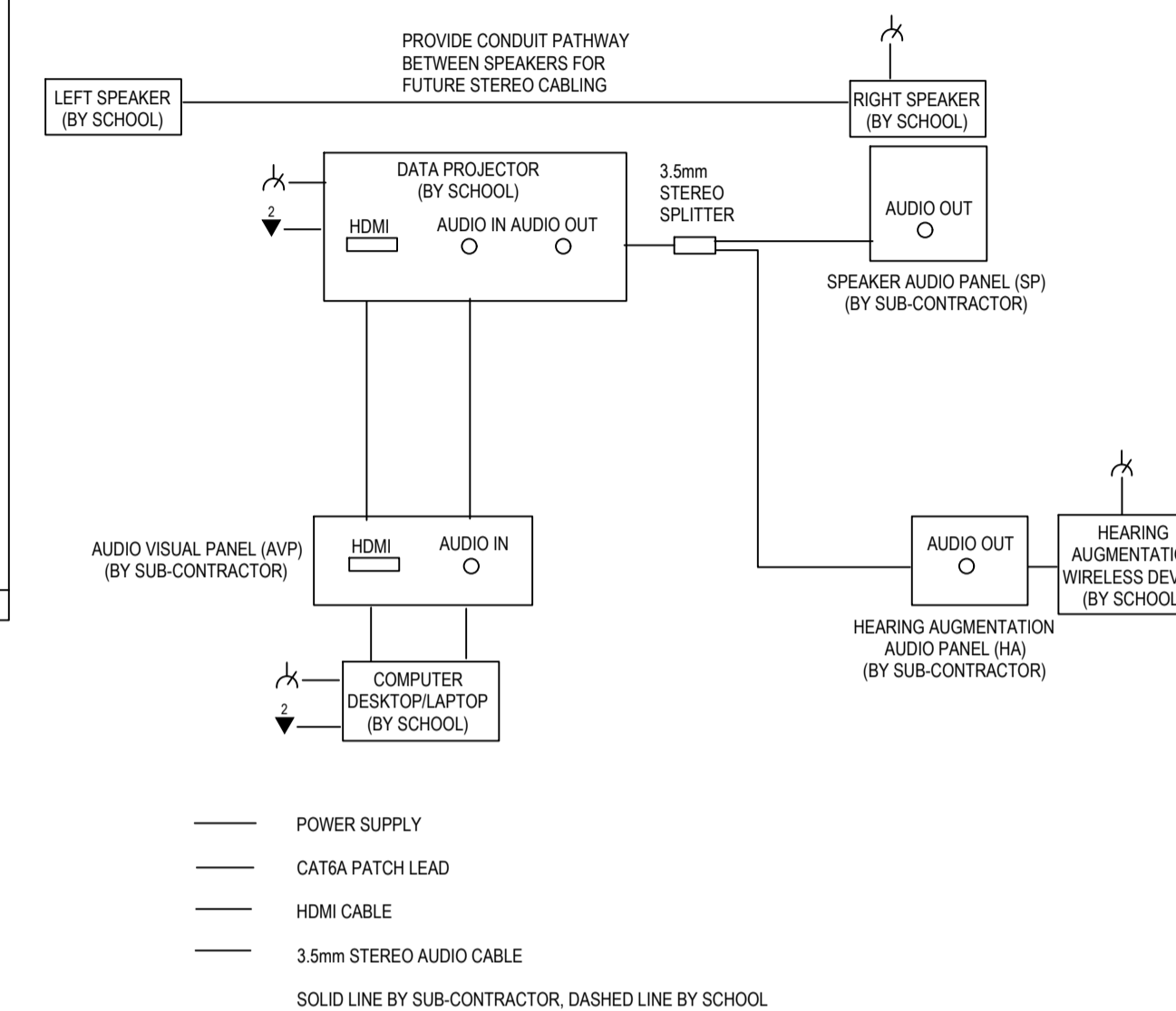
TYPICAL GLA AUDIO VISUAL SCHEMATIC
