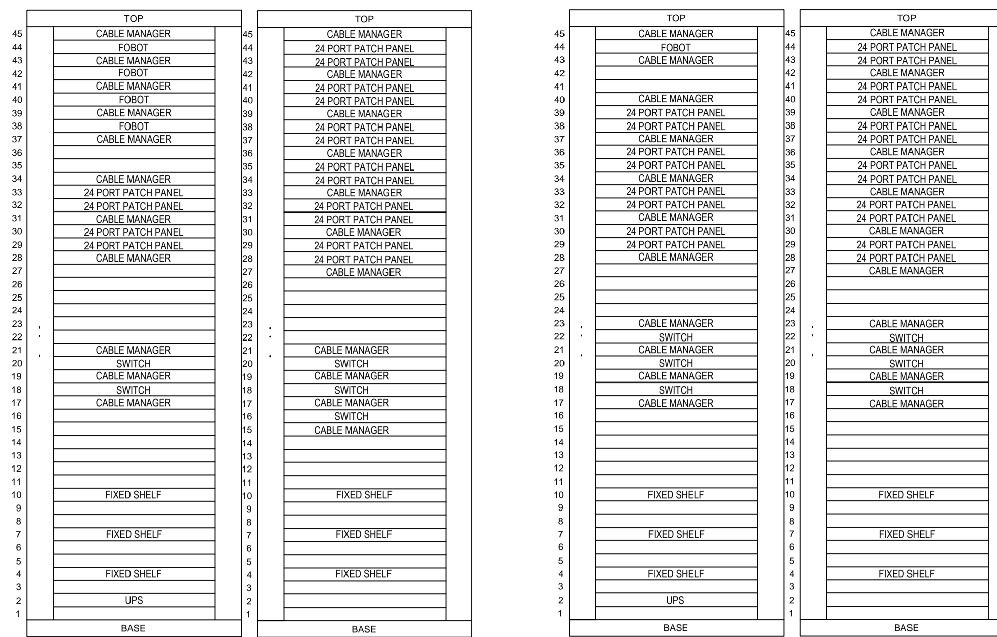
BD-GSC BD-G TYPICAL COMMUNICATIONS RACK LAYOUTS
