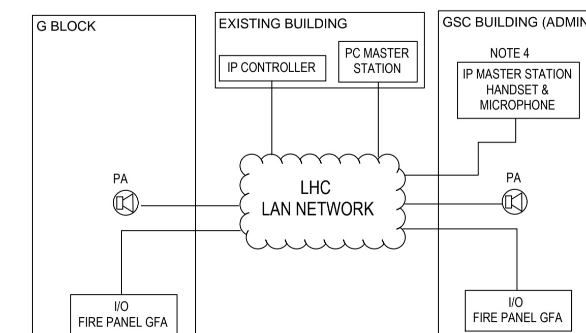
PUBLIC ADDRESS AND SCHOOL BELL SCHEMATIC
