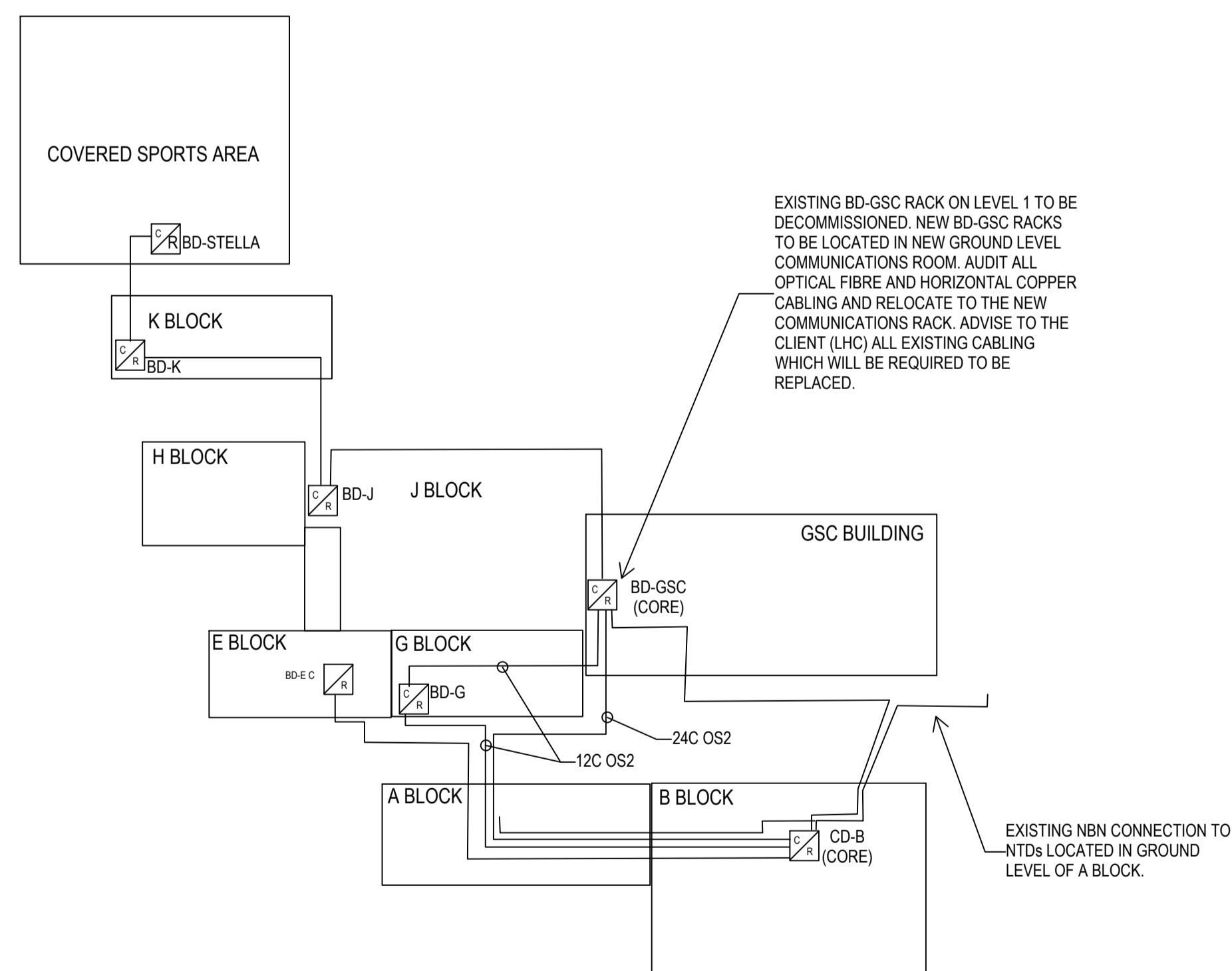
NEW OPTICAL FIBRE COMMUNICATIONS SCHEMATIC
